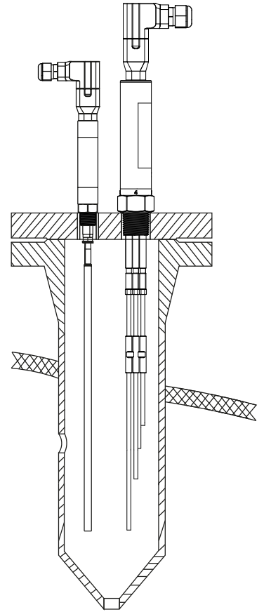
Figure 4 : Installation example 2, combination with self monitoring low level alarm probe SMLD 1000
