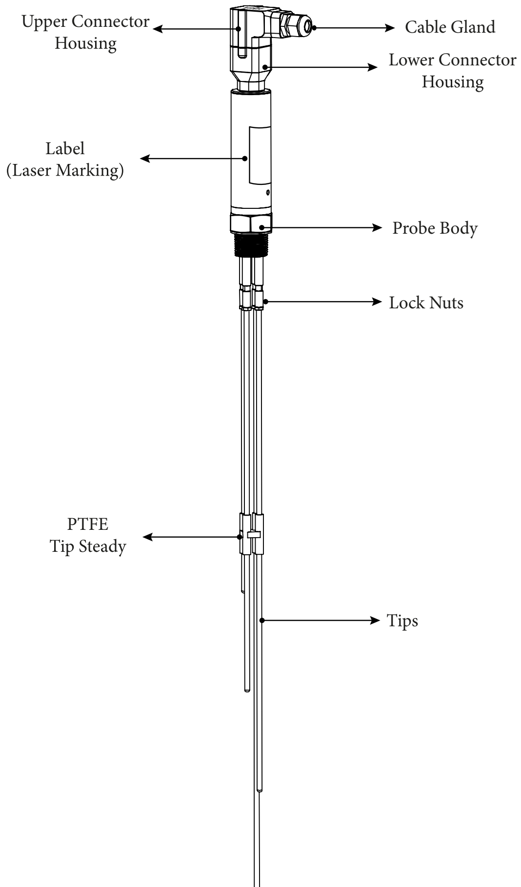
Figure 2 : Material description of SD 2400
