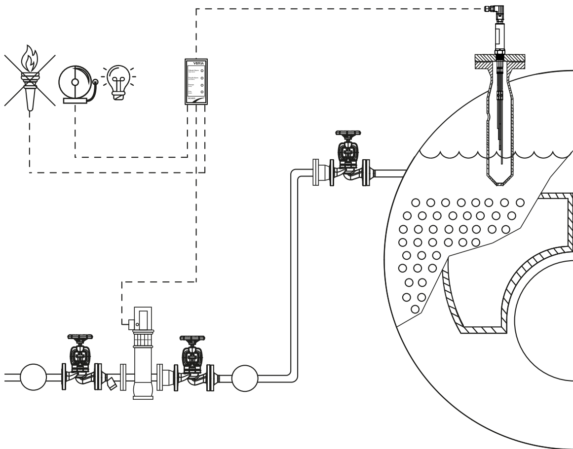
Figure 1 : SK 2000 System Application
