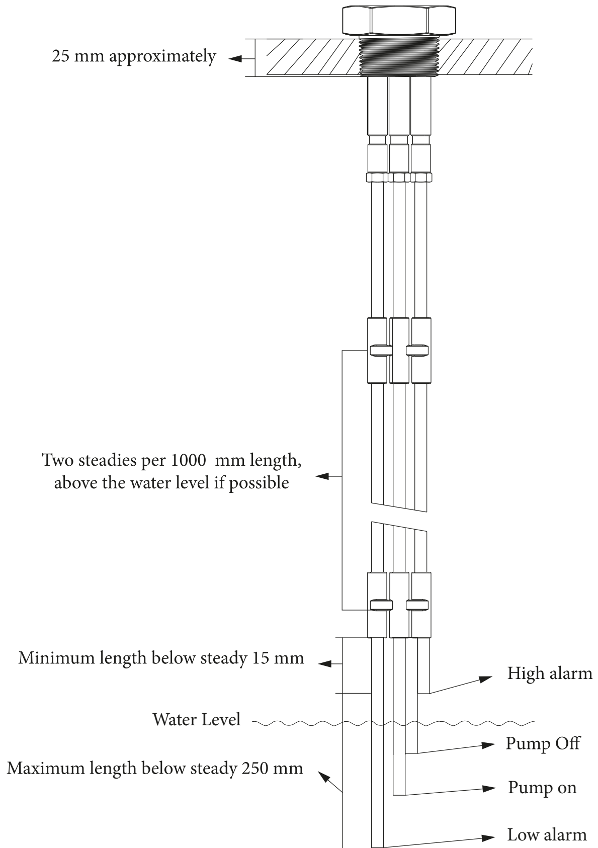
Figure 6 : Electrode length indication
