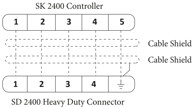
Figure 8 : Wiring diagrams
